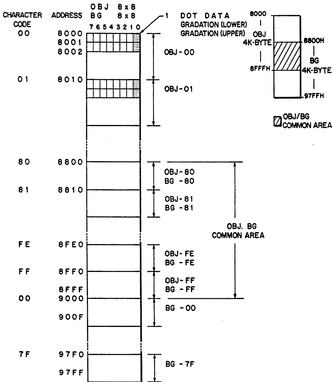
FIG. 13 CHARACTER RAM
